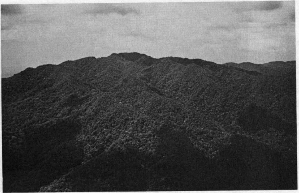
PLATE 4-23 Crocker Association in the Crocker Range
