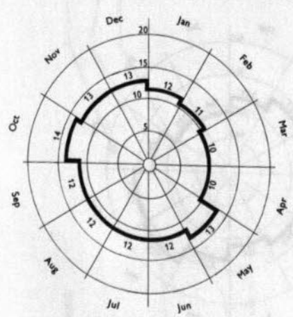
Keningau Mean Annual Raindays 142
