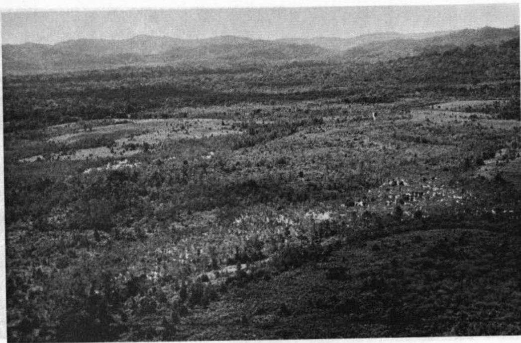
PLATE 4-13 Sook Association in the east of the Sook Plain with poorly drained remains of former lakes and river terraces
