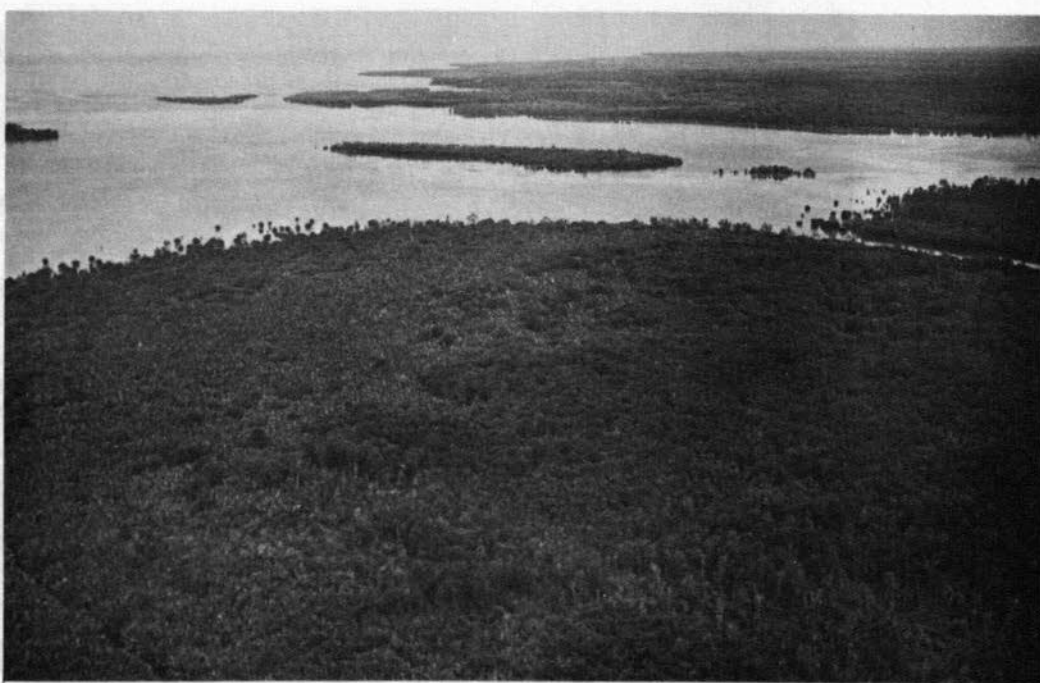
PLATE 4-4 Mangrove and nipah swamps (Weston Association) at Kuala Padas
