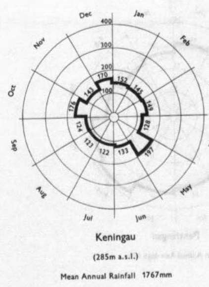
FIGURE 4-3 Mean monthly rainfall (mm)
