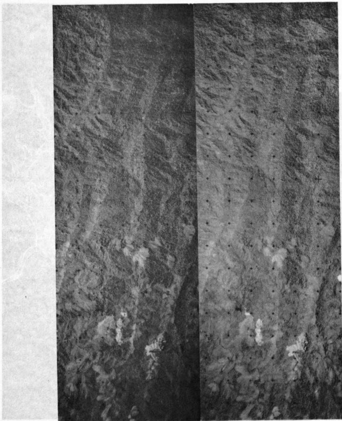
STEREOGRAM 4-1 The Crocker Range (Crocker Association) in the south of the Tenom District (Scale 1 : 64 000)
