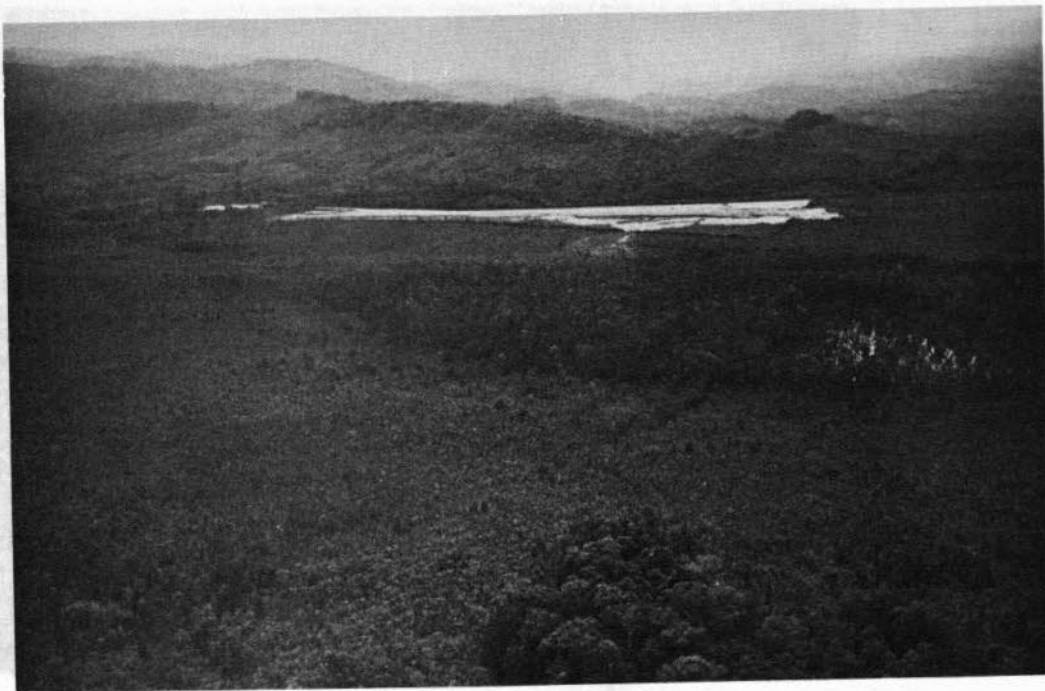
PLATE 4-17 Sipitang airfield. Extensive areas of Podzols (Kepayan Association) with peat swamp (Sipitang Association) at right. Sandstone and mudstone hills of the Lokan Association in the background
