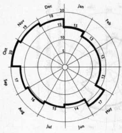
Sipitang Mean Annual Raindays 191
