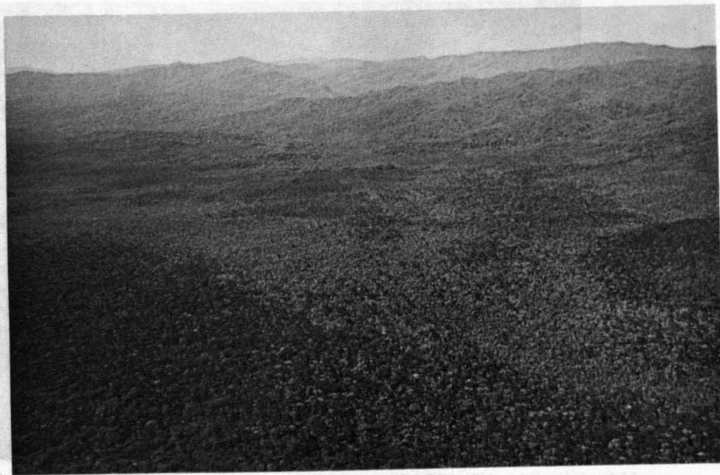
PLATE 4-18 Ulu Maligan. High altitude swamp (Sipitang Association) with Histosols under dark-toned vegetation and Podzols under pale vegetation. Mountains of the Maliau Association in the background
