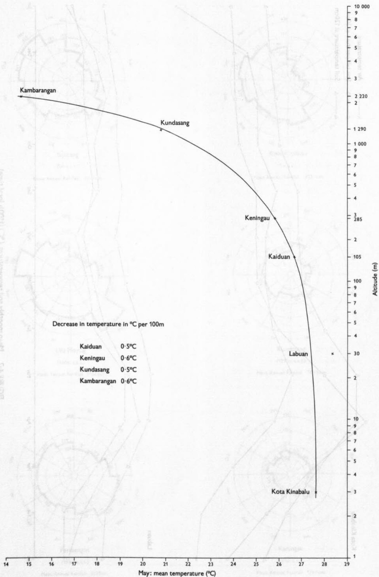
FIGURE 4-1 Decrease of temperature (°C) with altitude (m)
