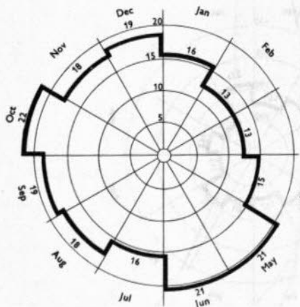
Ulu Moyog Mean Annual Raindays 205
