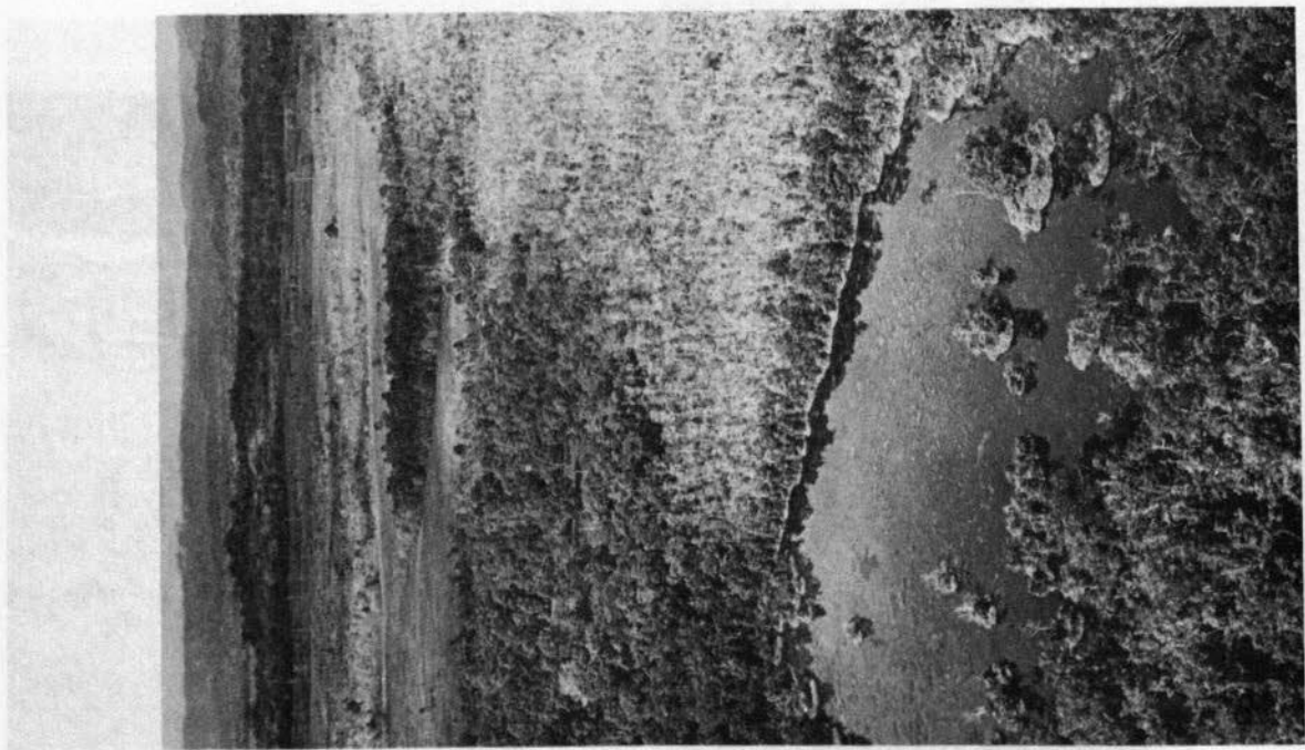
PLATE 4-15 Sook Plain. Kepayan Association under heath forest with Brantian Association (mainly under bracken) in the middle distance
