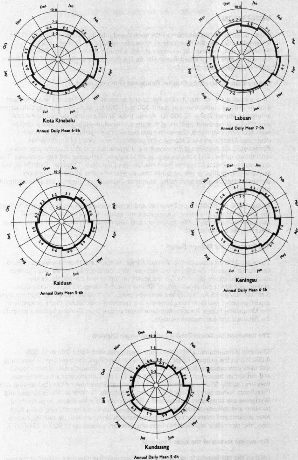
FIGURE 4-5 Mean daily sunshine (h)
