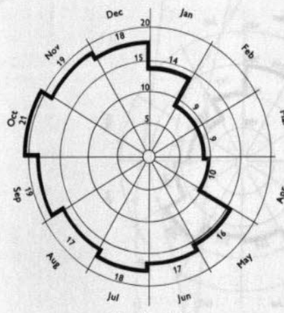
Kota Kinabalu Mean Annual Raindays 186
