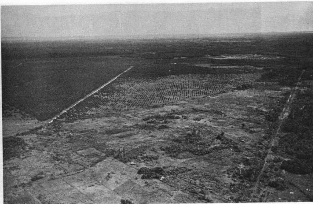
PLATE 4-9 Klias settlement scheme. Oil palm cultivation on peat (Klias Association)
