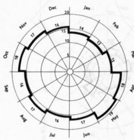
Pensiangan Mean Annual Raindays 196
