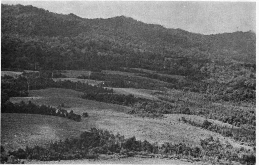
PLATE 4-12 The Brantian Association in the Sook Plain. Orthic Acrisols and Orthic Ferralsols under bracken with Gleyic Podzols under heath forest in the gullies
