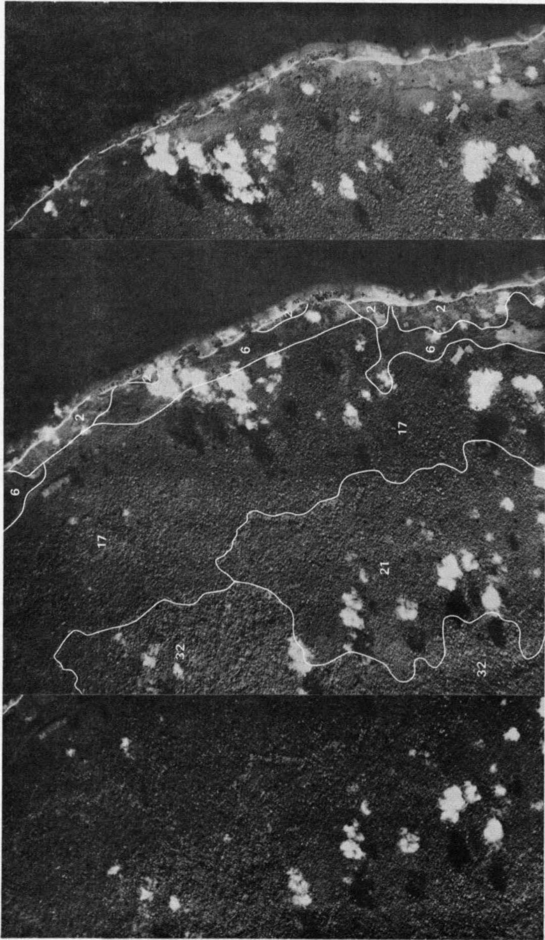
STEREOGRAM 2-12 East coast of the Dent Peninsula. The Semporna Association (21) on low limestone hills and the Tungku Association (17) on coastal plain of alluvium overlying coral. Coastal swamps of the Sapi Association (6) lie inland from the coastal beaches of the Usukan Association (2). The Tengah Nipah Association (32) is on moderate hills of sandstone and mudstone (Scale 1 : 57 000)
