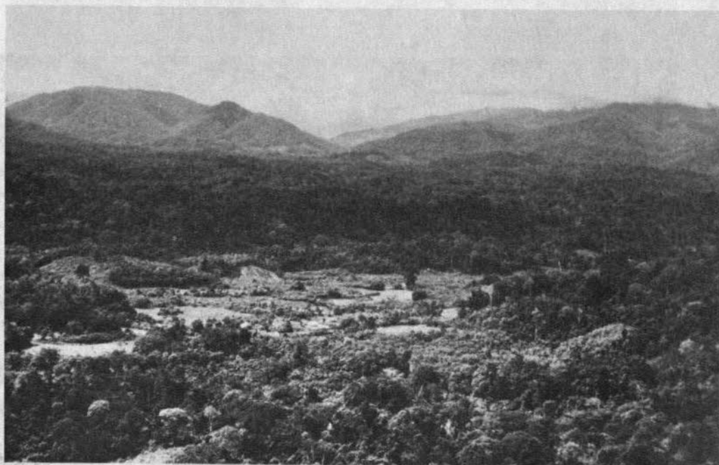
PLATE 2-23 The Sungai Tongod south of Kuala Mananam. Low terraces of the Karamuak Association with low hills of the Dalit Association and mountains of the Mentapok Association in the background
