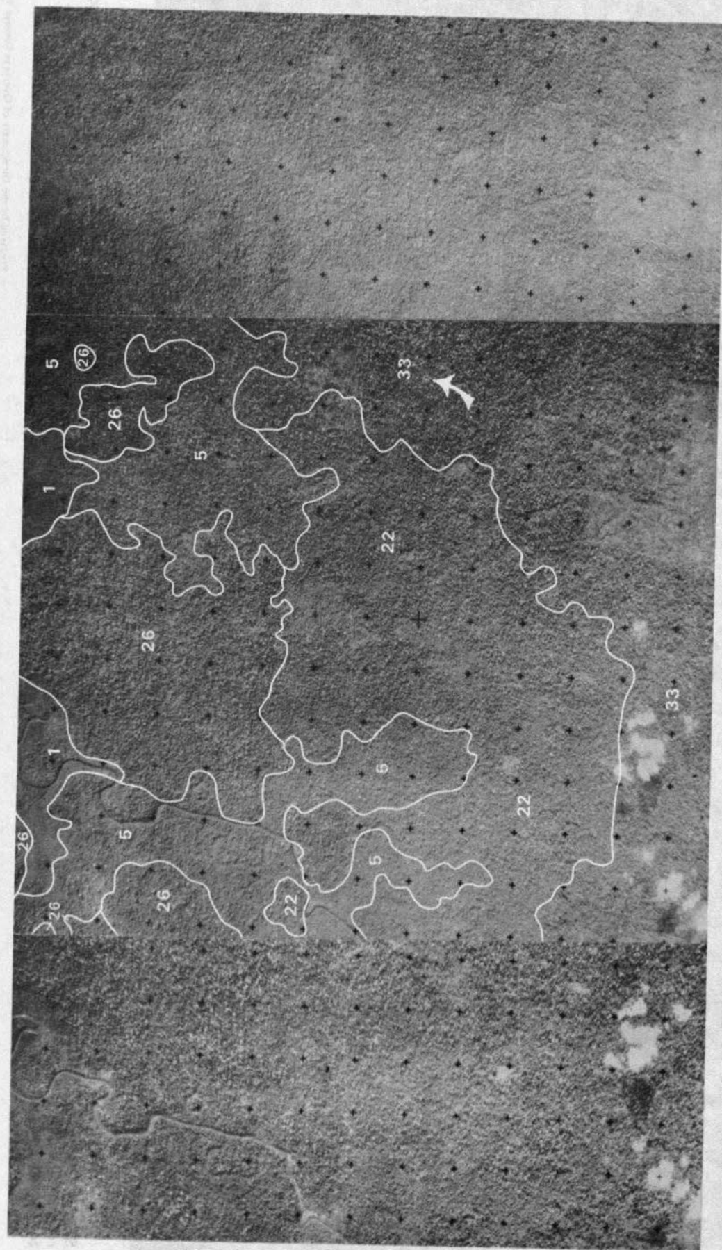
STEREOGRAM 2-8 Kretam. The Kretam (33), Rumidi (26) and Lungmanis (22) Associations on slump formations lacking clearly defined patterns of relief and drainage; mud volcano (arrowed) seen as a small clearing on the summit of a low circular hill. The floodplain of the Kretam and its tributaries are in the Kinabatangan Association (5) and coastal swamps are in the Weston Association (1) (Scale 1 : 54 000)
