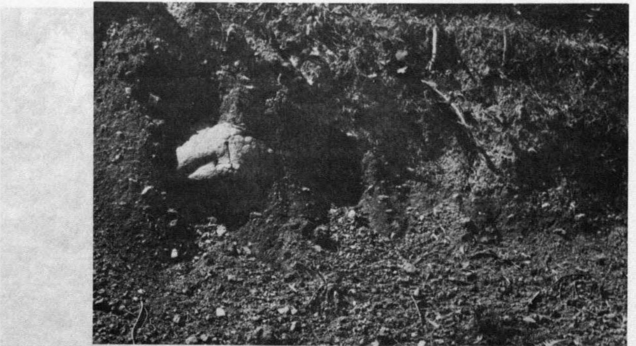
PLATE 2-10 Garinono Formation near Ulu Dusun
