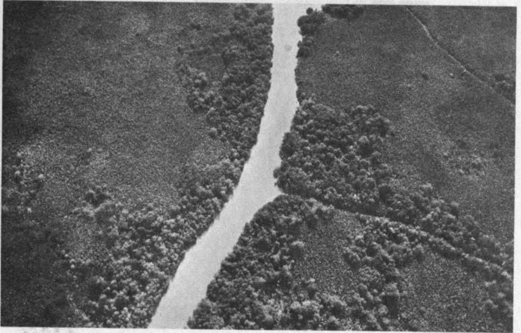
PLATE 2-11 Segama estuary. Coastal swamps of nipah palm ( Nypa fruticans ) with mangrove species bordering rivers
