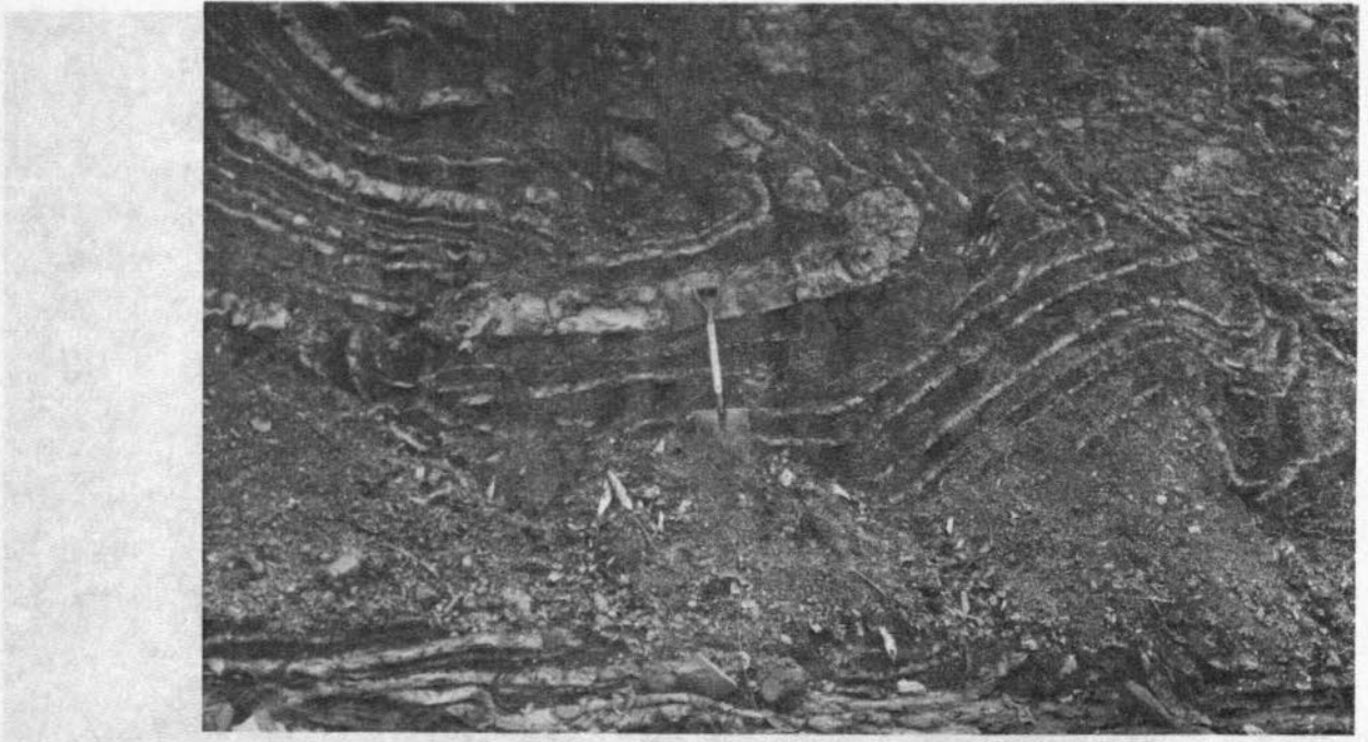
PLATE 2-9 Interbedded sandstone and shale of the Kulapis Formation producing mixed regolith at upper right
