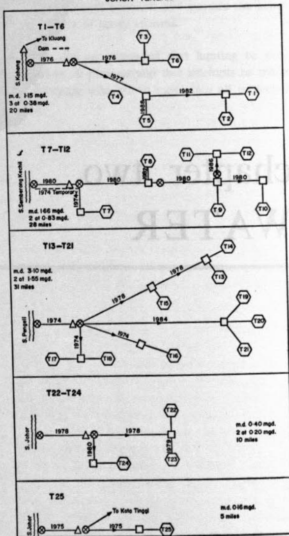
SCHEMATIC VILLAGE WATER SUPPLY JOHOR TENGAH
