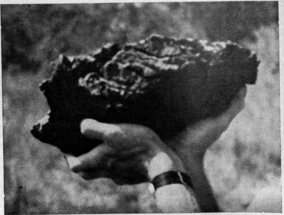
Large "lenticle" of clay from the subsoil of Muhoroni clay loam. Note curved cracks outlining smaller lenticles. The shaded lower surface and the back of the lenticle of clay have slickenside surfaces that intersect at the right.
