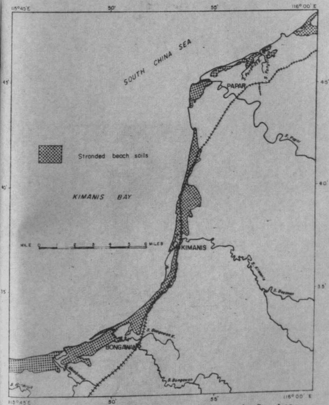
Fig. 2. Distribution of stranded beach soils. Kimanis Bay Area
