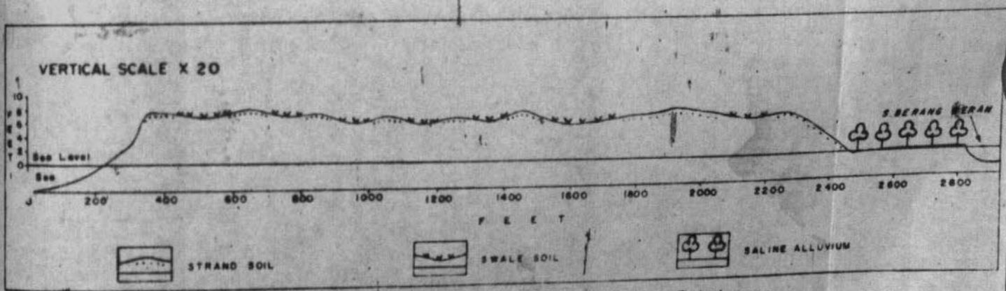
Fig 1. Section showing the micro-topography of a stranded beach soil, Kota Belud area.
