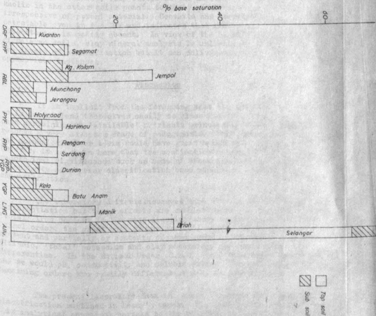
FIG. 3(b) % BASE SATURATION
