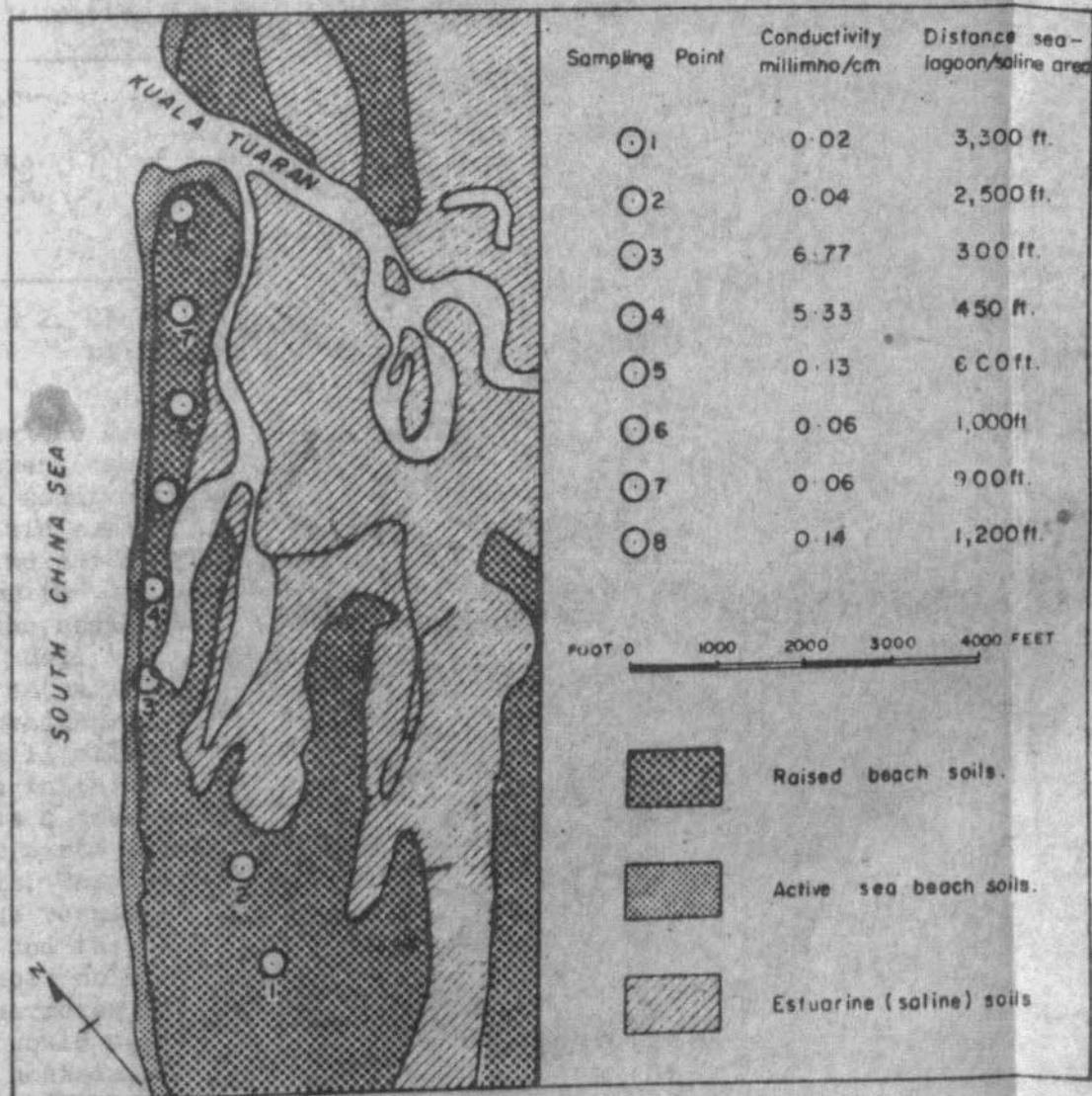
Fig3. Conductivity of ground waters in a stranded beach formation, Tuaran area.
