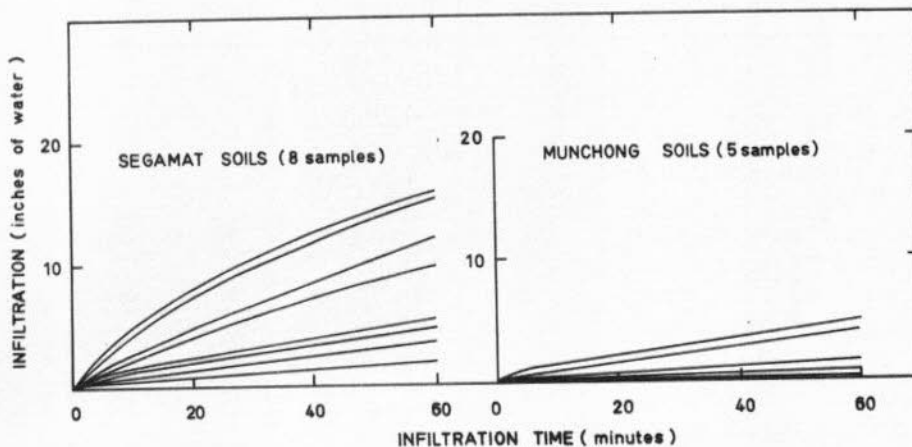
Figure 7-7 Infiltration Rates
